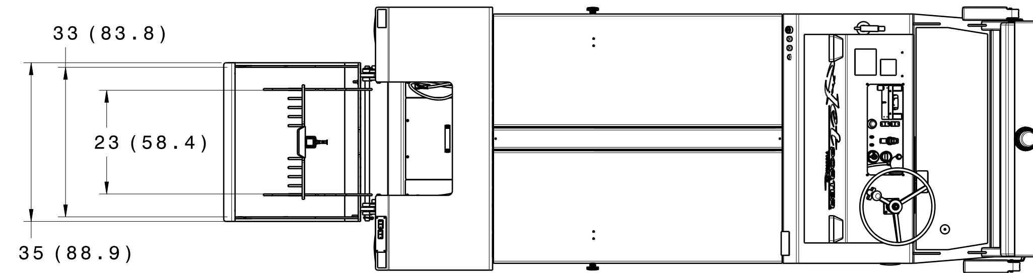
TOP VIEW
