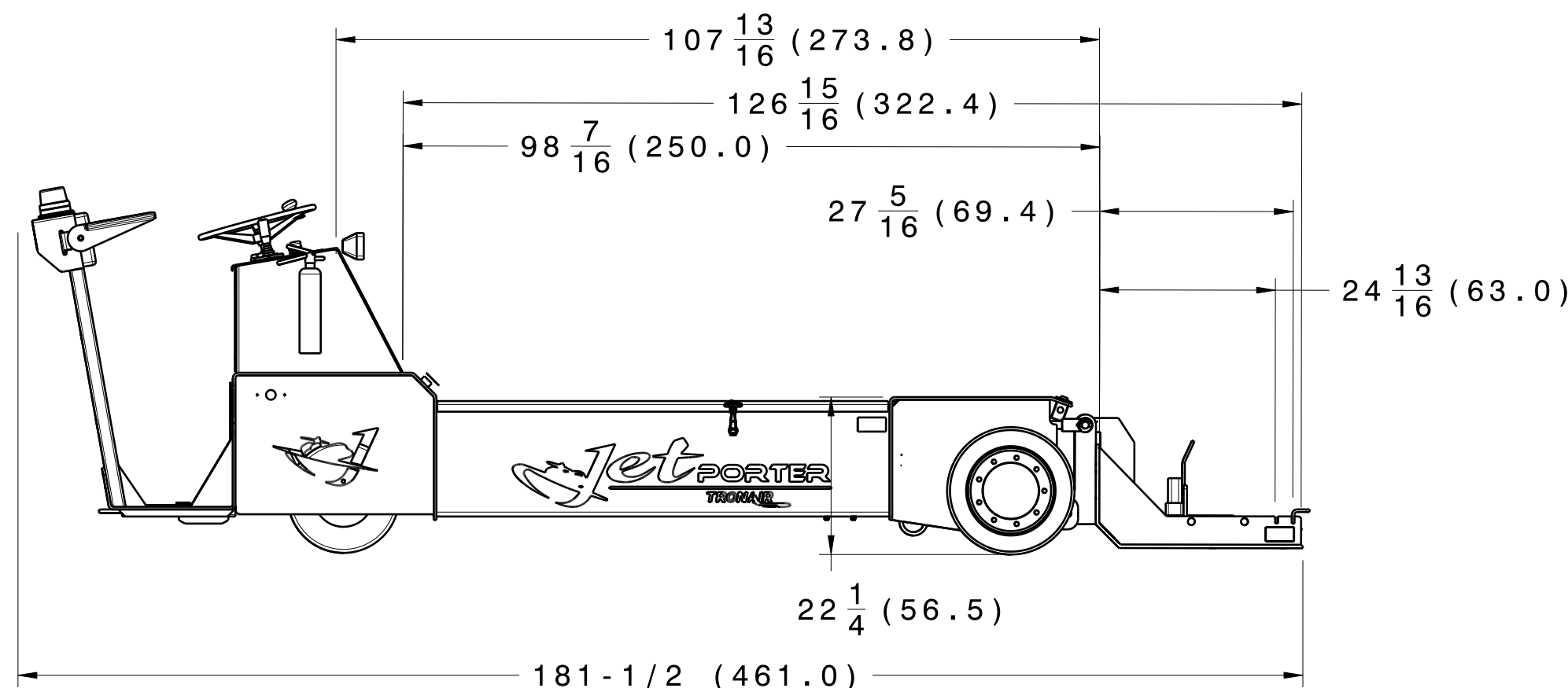
RIGHT SIDE VIEW 181-1/2 (461.0)
